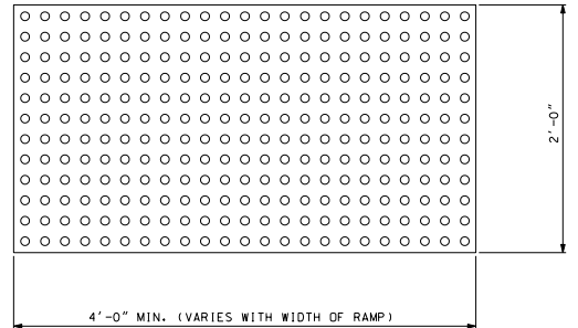
TRUNCATED DOME PLAN VIEW
