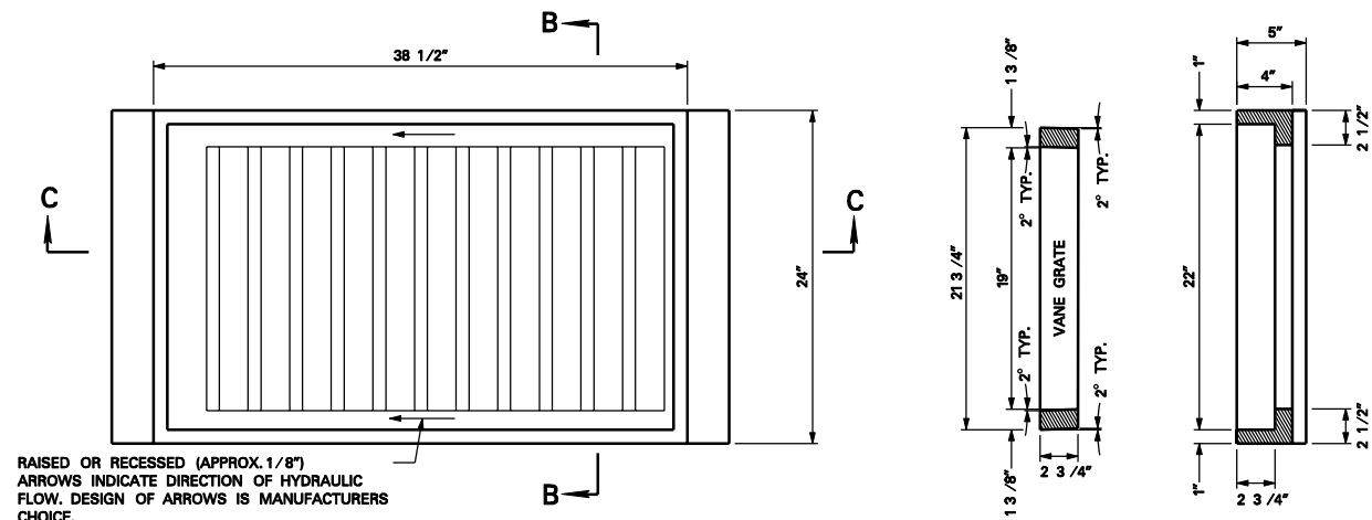
PLAN VIEW
