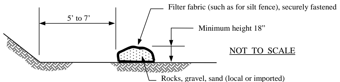
Figure ES-17-1 Rock Filter Berm
